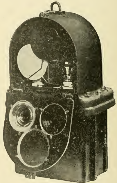
Fig. 216. Signal Box with Front Cover Down
